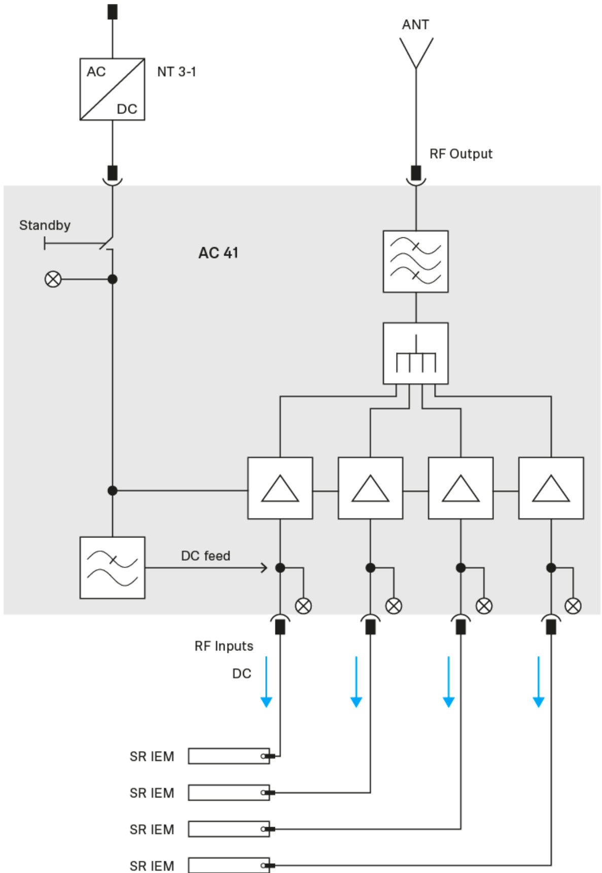
Block diagram AC 41
